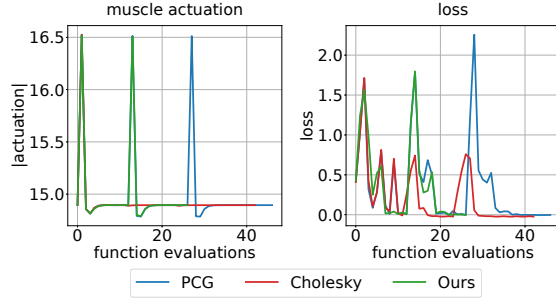
Fig. 5. The progress of running L-BFGS optimization to solve the “Torus” example. The horizontal axis shows the number of function evaluations used, and the vertical axes plot the magnitude of the actuation (left) and loss (right).
