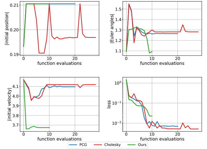
Fig. 3. The progress of running L-BFGS optimization to solve the “Bunny” example. The horizontal axis shows the number of function evaluations used, and the vertical axes plot the lengths of the initial position (top left), initial Euler angles (top right), initial velocity (bottom left), and loss (bottom right).
